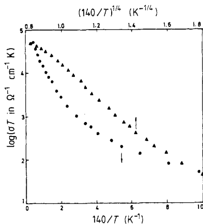
Figure 7. The variation of \log(\sigma T) with (140/T) and (140/T)^{-1/4} for Y_2Mo_2O_7 .
