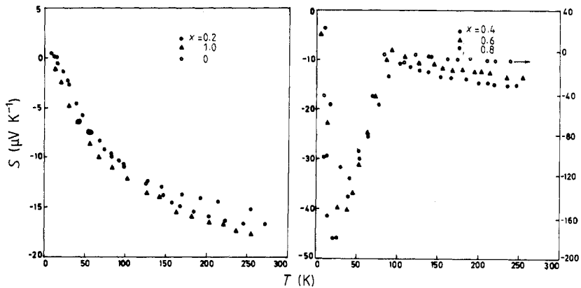
Figure 4. The variation of the thermoelectric power, S , with temperature for (Dy_xY_{1-x})_2Mo_2O_7 .
