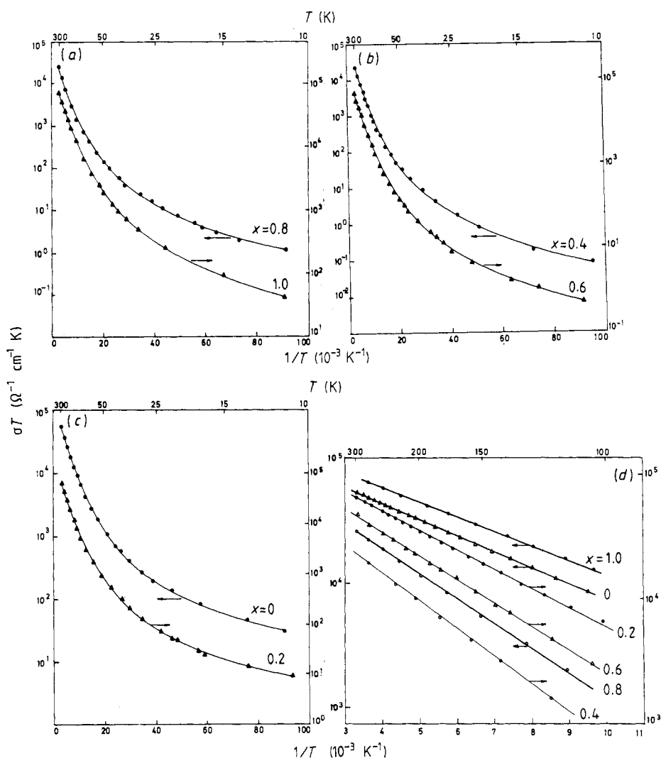
Figure 1. Plots of \log(\sigma T) versus reciprocal temperature for (\text{Dy}_x\text{Y}_{1-x})_2\text{Mo}_2\text{O}_7 .
