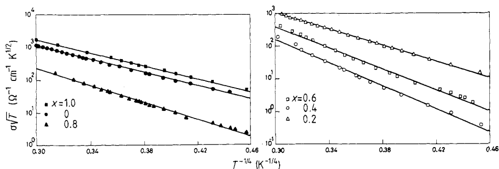
Figure 3. Plots of \log(\sigma\sqrt{T}) versus T^{-1/4} for (\text{Dy}_x \text{Y}_{1-x})_2 \text{Mo}_2 \text{O}_7 .
