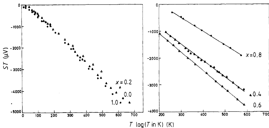
Figure 6. Plots ST versus T \log(T) for (Dy_xY_{1-x})_2Mo_2O_7 .
