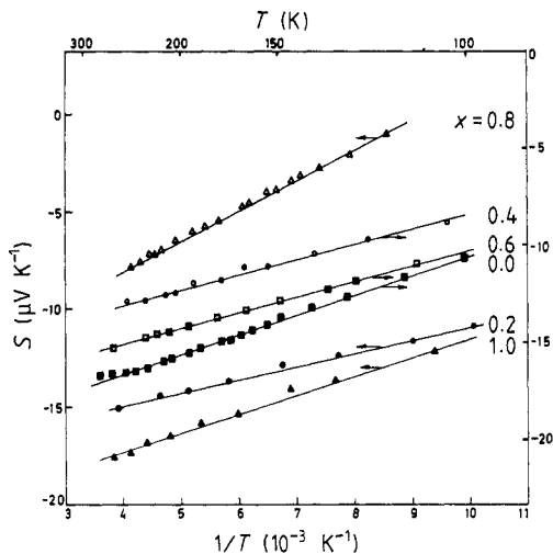
Figure 5. Plots of the thermoelectric power, S , versus reciprocal temperature for (\text{Dy}_x \text{Y}_{1-x})_2 \text{Mo}_2 \text{O}_7 .
